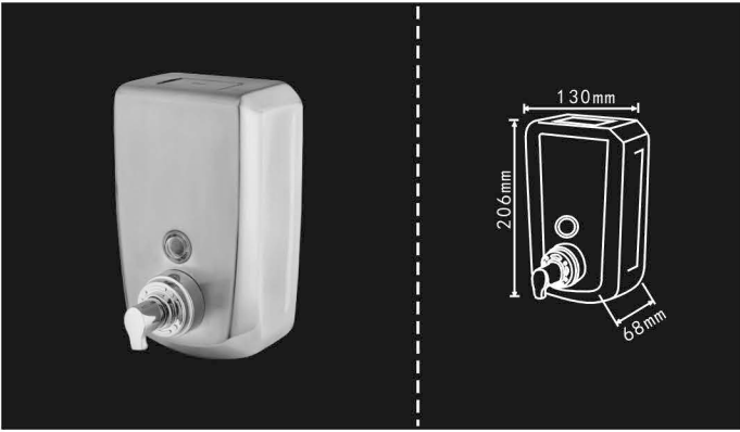
SFH9-1200ABF Capacity: 1200ml Material: 304# Stainless steel Surface: Mirror polish & satin finish Using the 1230D pump With a lock Qty/Ctn: 20pcs G.W./N.W.: 15.5kgs/12kgs Size/Ctn: 65.5*27*45cm
