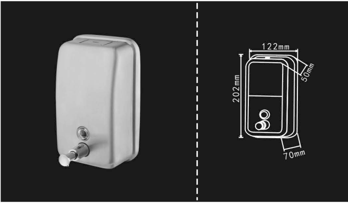
SF H5-1000BF Capacity: 1000ml Material: 304# Stainless steel Surface: Satin finish With a lock Using the 1230B pump Qty/Ctn: 20pcs G.W./N.W.: 14kgs/10.6kgs Size/Ctn: 65.5*27*43cm
