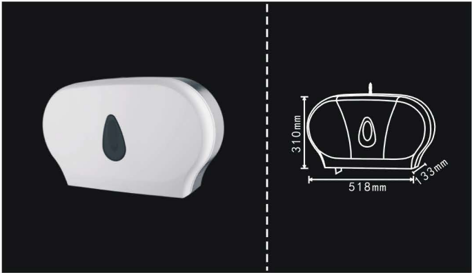
SF-P8012A Material: ABS Plastic With a lock Qty/Ctn: 8 pcs G.W./N.W.: 16.4kgs/11.2kgs Size/Ctn: 57.7*53.8*66cm
