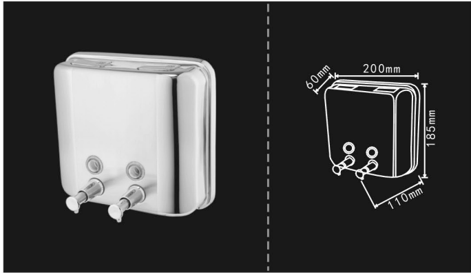
SFH15-1500AB Capacity: 1500ml Material: 304 Stainless steel Surface: Mirror polish & satin finish Qty/Ctn: 20pcs G.W./N.W.: 20kgs/16kgs Size/Ctn: 63*43*41cm
