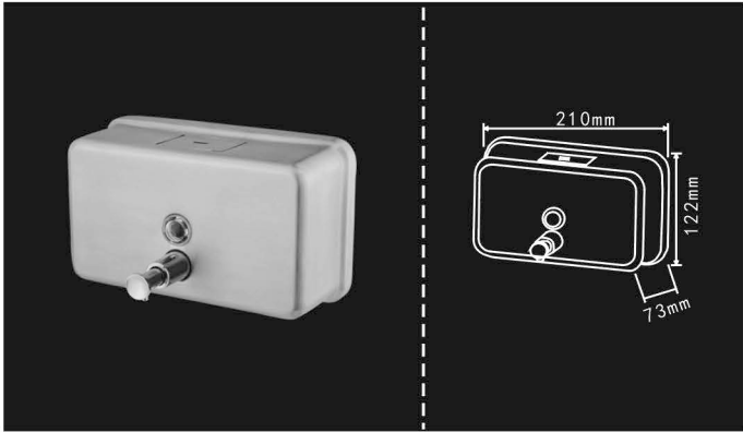
SF H11-1300BHFT Capacity: 1200ml Material: 304# Stainless steel Surface: Satin finish With a lock Using the 1230T pump With a plastic container inside Qty/Ctn: 20pcs G.W./N.W.: 18.5kgs/15kgs Size/Ctn: 65.5*27*45cm
