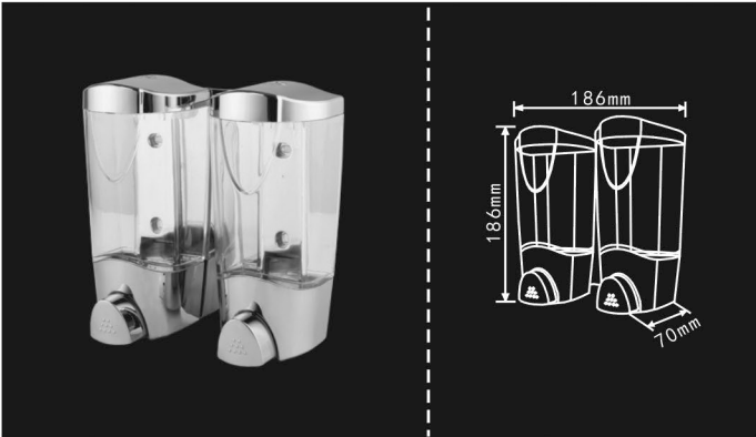
SF-450BD Capacity: 2×450 ml Material: ABS plastic cover (chrome plated) with AS plastic bottle Qty/Ctn: 24 pcs G.W./N.W.: 15.5kgs/11kgs Size/Ctn: 59.6*36*41.3cm
