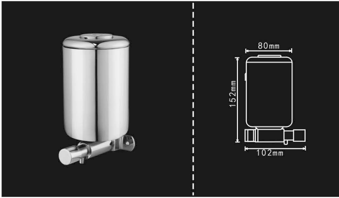
SF H10-500A Capacity: 500ml Material: Brass Surface: Chrome finish With no lock Qty/Ctn: 30pcs G.W./N.W.: 18.5kgs/14.9kgs Size/Ctn: 49*39*35.5cm
