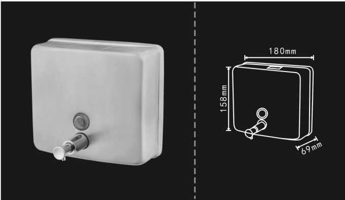
SFH13-800B Capacity: 800ml Material: 304 Stainless steel Surface: Satin finish Versions: Liquid/Spray Qty/Ctn: 24pcs G.W./N.W.: 23.6kgs/18.5kgs Size/Ctn: 68*57*35cm
