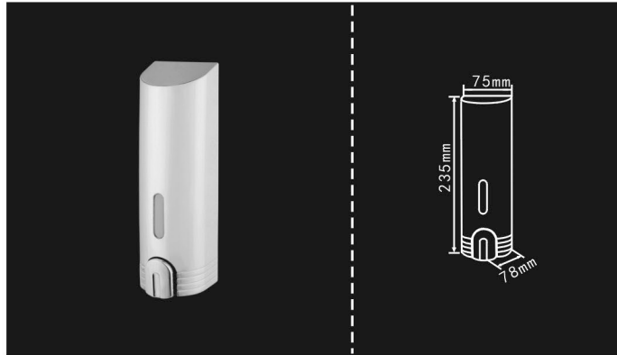
SF-400B Capacity: 400ml Material: ABS plastic cover (chrome plated) with PE plastic bottle Qty/Ctn: 50pcs G.W./N.W.: 18.5kgs/14.5kgs Size/Ctn: 46*47*52cm
