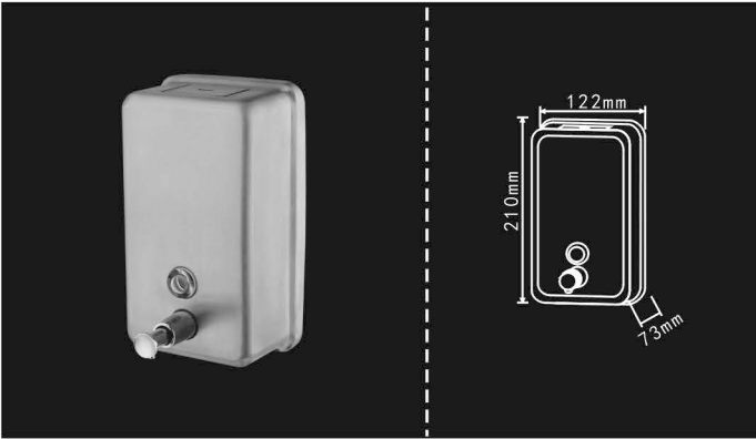
SFH11-1300BFT Capacity: 1200ml Material: 304# Stainless steel Surface: Satin finish With a lock Using the 1230T pump With a plastic container inside Qty/Ctn: 20pcs G.W./N.W.: 18kgs/14.6kgs Size/Ctn: 65.5*27*45cm
