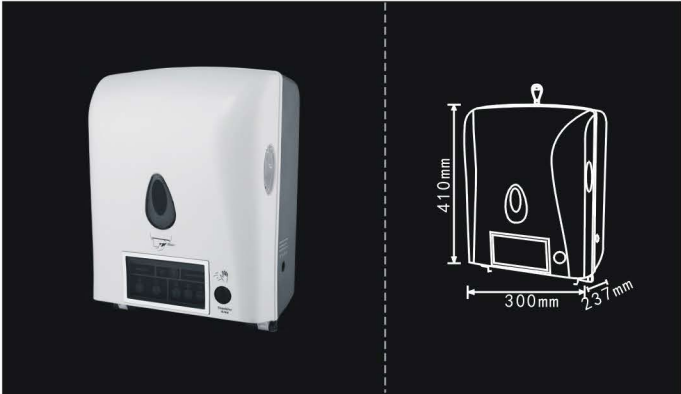
SF-P8388A Material: ABS Plastic Characteristics: Sensor paper dispenser With a lock Qty/Ctn: 4 pcs G.W./N.W.: 15.6kgs/11.3kgs Size/Ctn: 65.5*44.3*55cm
