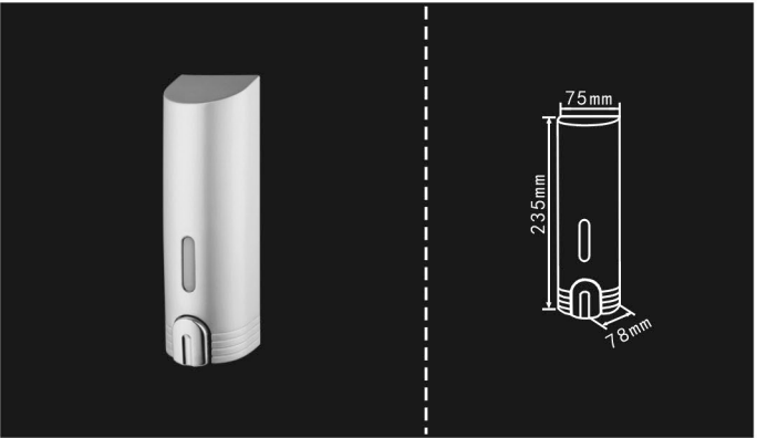
SF-400S Capacity: 400ml Material: ABS plastic cover (spray argentite paint) with PE plastic bottle, the button is chrome plated Qty/Ctn: 50pcs G.W./N.W.: 18.5kgs/14.5kgs Size/Ctn: 46*47*52cm
