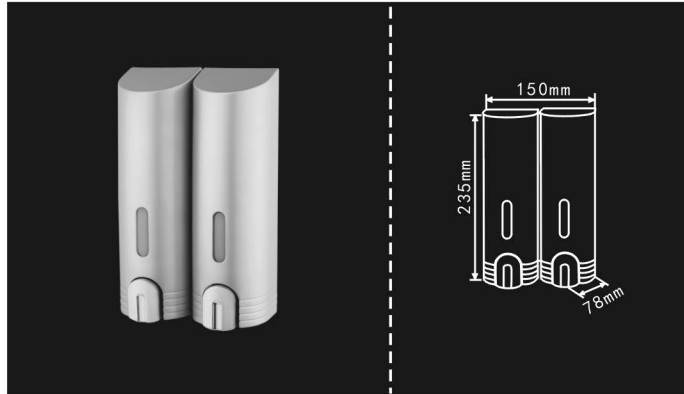
SF-400SD Capacity: 2×400ml Material: ABS plastic cover (spray argentite paint) with PE plastic bottle, the button is chrome plated Qty/Ctn: 30pcs G.W./N.W.: 20.8kgs/17.5kgs Size/Ctn: 50*49*52cm
